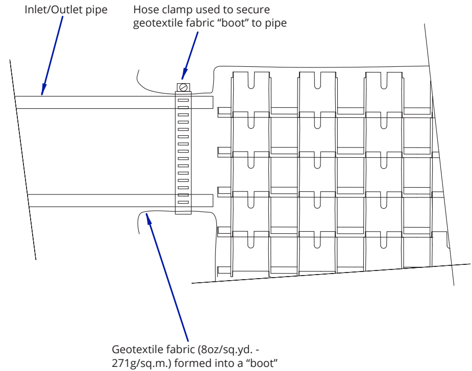
SIDE VIEW
